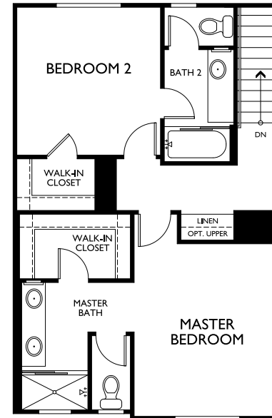
THIRD FLOOR
